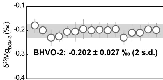
Figure S-6 Long-term variations in the magnesium isotope composition of rock standard BHVO-2, indicating a reproducibility of 0.027 ‰ (2 s.d.).
