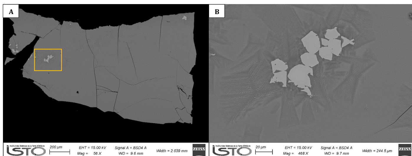
Figure S-1 (a) Grain from EXP06B with localized quench crystals. (b) Detail from (a) showing the dendrites and spinel crystals produced during quench.
