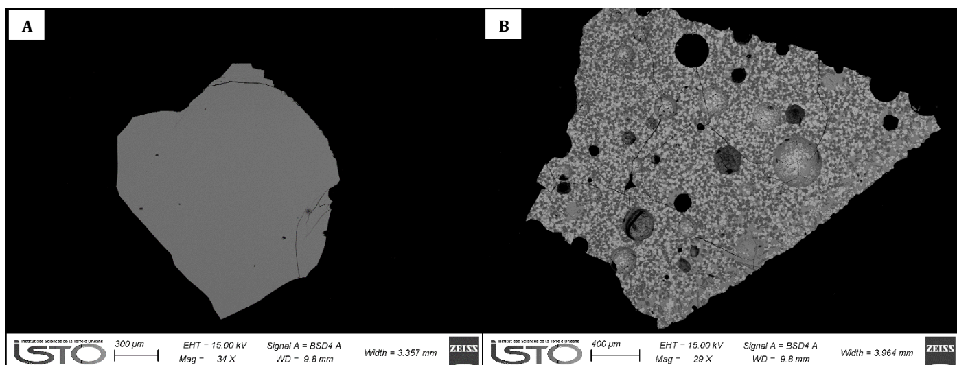
Figure S-2 (a) Homogeneous glass from EXP07. (b) Grain from EXP07 with olivine and spinel crystals produced during the experiment.
