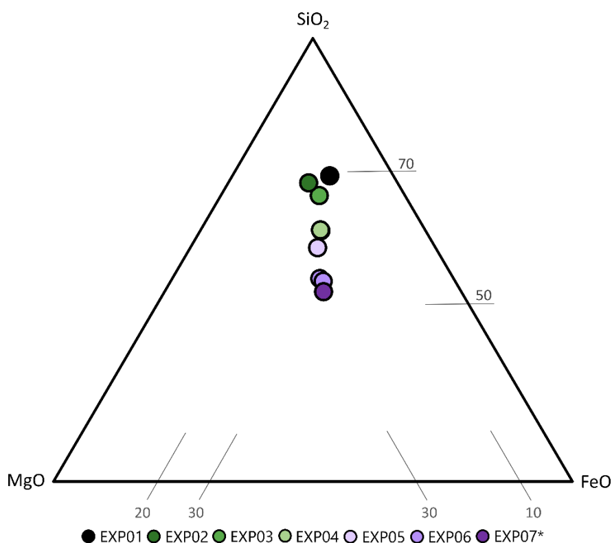
Figure S-3 Chondrites ternary diagram (Lodders and Fegley Jr, 2015) with compositional range of experimental glasses.
