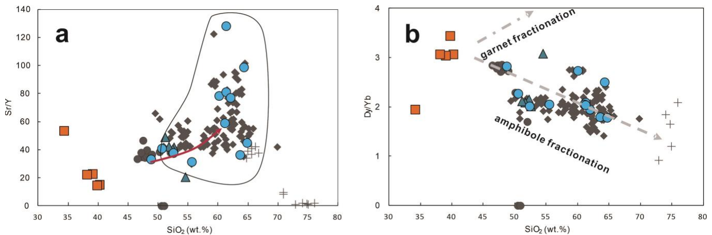
Figure S-4 Trace element signature of cumulate, mafic magmas (121-124 Ma) and ore-forming magmas (136-145 Ma). (a) fields of barren vs. porphyry Cu ± Au ± Mo productive magmas are from Loucks (2014); the arrow shows the predicted fractionation trend for crystallization of 50 wt. % amphibole ( D_{Sr}^{amph/melt} = 0.60 ; D_{Y}^{amph/melt} = 1.2 ; D_{SiO_2}^{amph/melt} = 0.80 ), 40 wt. % clinopyroxene ( D_{Sr}^{cpx/melt} = 0.13 ; D_{Y}^{cpx/melt} = 0.80 ; D_{SiO_2}^{cpx/melt} = 1.0 ) and 10 wt. % magnetite ( D_{Sr}^{mgt/melt} = 0 ; D_{Y}^{mgt/melt} = 0 ; D_{SiO_2}^{mgt/melt} = 0 ); (b) Garnet versus amphibole fractionation trends are from Davidson et al. (2007).
