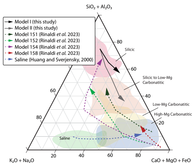
Figure 3 Ternary diagram comparing predicted model fluid compositions (curves and arrows) with high density fluid (HDF) compositions in fibrous diamonds (coloured fields from Weiss et al. , 2022). Solid curves and arrows show fluid evolution paths predicted by DEW models from this study (Models I and II). Dashed curves and arrows show paths from Rinaldi et al. (2023), and Huang and Sverjensky (2020). Models I and II trajectories reproduce the transition from silicic to carbonatitic compositions and overlap natural HDF arrays. The simulations of Rinaldi et al. (2023) represent reactions between fluids of different initial compositions (eclogitic, silicic, transitional silicic-carbonatitic, and carbonatitic) and mantle lithologies including carbonated peridotite (Models 151 and 152) and eclogite or websterite (Models 154 and 158) and overlap numerous natural fluid inclusion trends. The model of Huang and Sverjensky (2020) describes the evolution of saline fluids as they mix and react with highly Mg-rich carbonatitic compositions.
