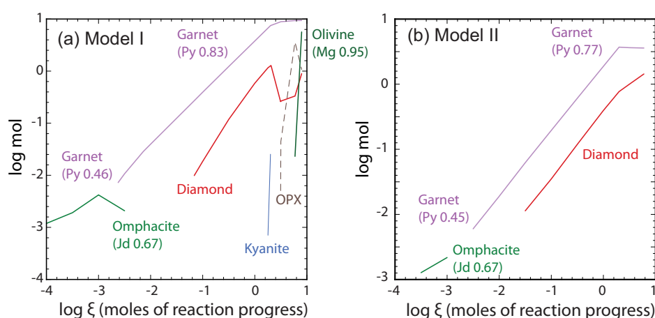
Figure 1 Predicted mineral precipitation during reaction progress in two DEW fluid-rock interaction models. Log mineral abundance (mol) is plotted against log reaction progress ( \xi ), where \xi represents the extent of fluid-rock interaction simulated by irreversible mass transfer in EQ6. (a) Model I predicts progressive garnet growth (Py 0.46–0.83), followed by omphacite (Jd ~0.67), diamond precipitation, and late olivine (Mg# ~0.95), with minor orthopyroxene and kyanite at advanced reaction progress. (b) Model II shows a simpler sequence dominated by garnet and omphacite formation followed by diamond precipitation. Values in parentheses indicate representative mineral compositions predicted by the models. The simulations illustrate mineral assemblages produced during mantle fluid-rock interaction capable of forming diamond bearing eclogitic-peridotitic assemblages.
